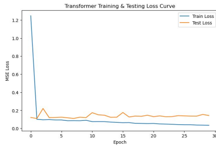
(c) Transformer Training and Testing loss Curve
