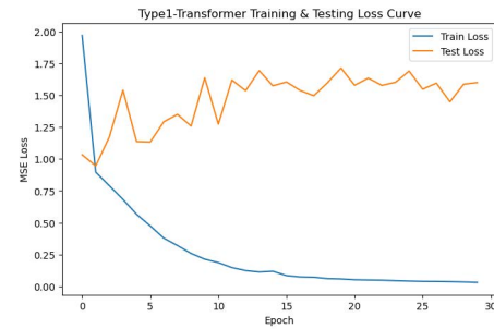
(d) Type1-Transformer Training and Testing loss Curve
